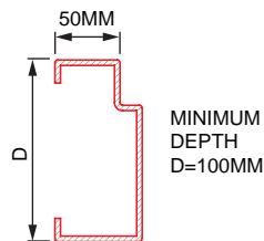
Frame: Single Rabbet
