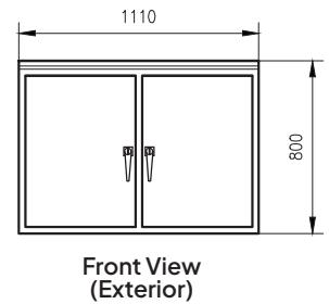
Fire Hose Cabinet
